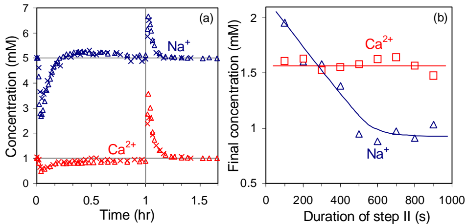
Fig. 3. Experimental data of ion-selectivity of porous electrodes in a capacitive deionization-cell, see Fig. 1. (a) Ion effluent concentration in a mixture of \text{NaCl} and \text{CaCl}_2 during adsorption at V_{\text{cell}}=1.2 V, and desorption after t=1 hr at V_{\text{cell}}=0 V. (b) Final ion concentrations obtained in recycle volume in the ion recovery-step III as function of duration of washing step II. Lines serve to guide the eye.
